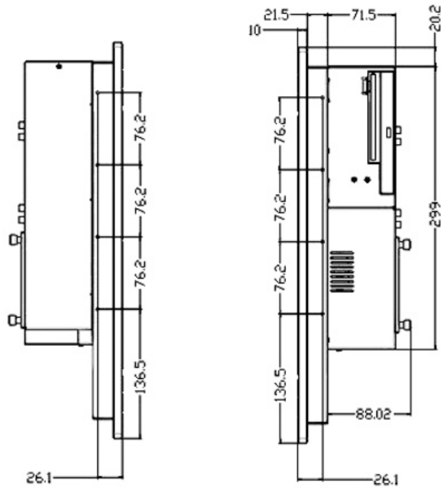
Figure 1-17: PPC-120 17" Left Side Diagram (mm)
