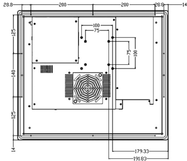
Figure 1-15: PPC-120 17" Rear Diagram (mm)
