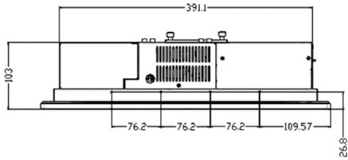
Figure 1-11: PPC-120 15" Top Diagram (mm)
