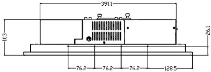
Figure 1-16: PPC-120 17" Top Diagram (mm)
