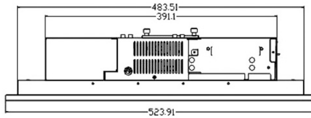
Figure 1-21 PPC-120 19" Top Diagram (mm)
