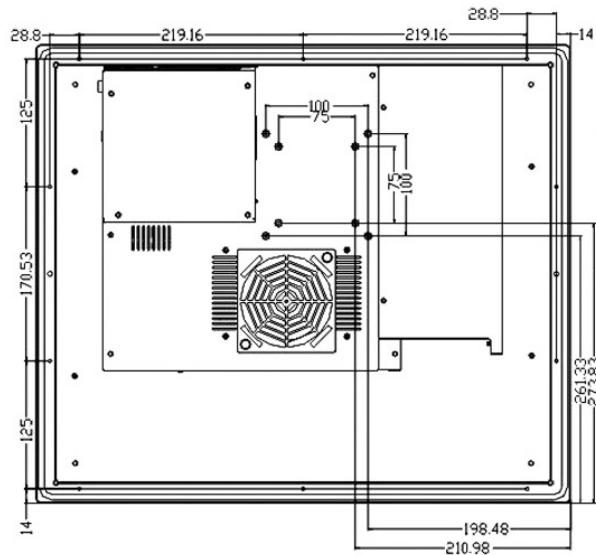
Figure 1-20: PPC-120 19" Rear Diagram (mm)
