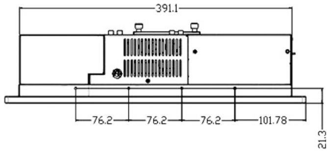
Figure 1-6: PPC-120 12" Top Diagram (mm)
