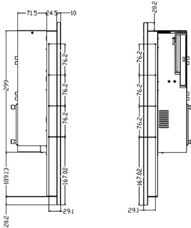
Figure 1-22: PPC-120 19" Left Side Diagram (mm)
